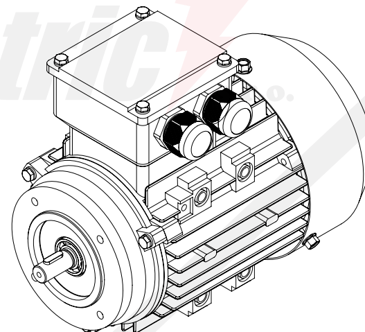
1AL-63-B14 Mounting diagram
